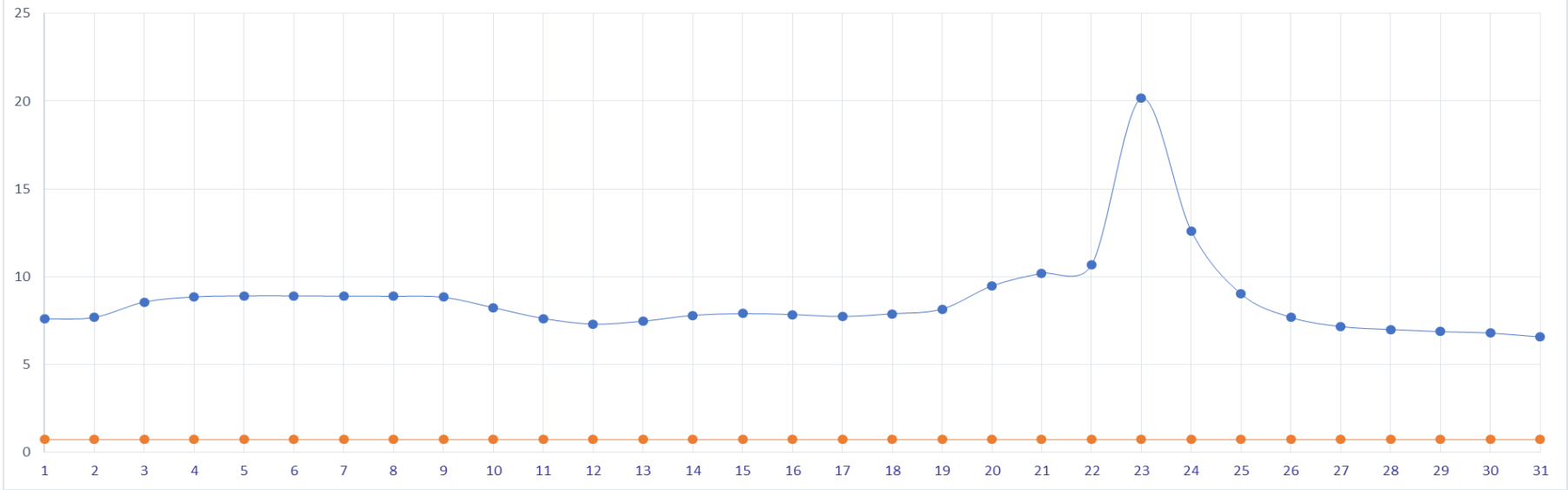
Didachara Environmental flow for Dec 2017 Required Flow - 0.715 m 3 /sec, Actual flow released - Day Average m 3 /sec Note : From 4th october 2017 plant is not in operations
