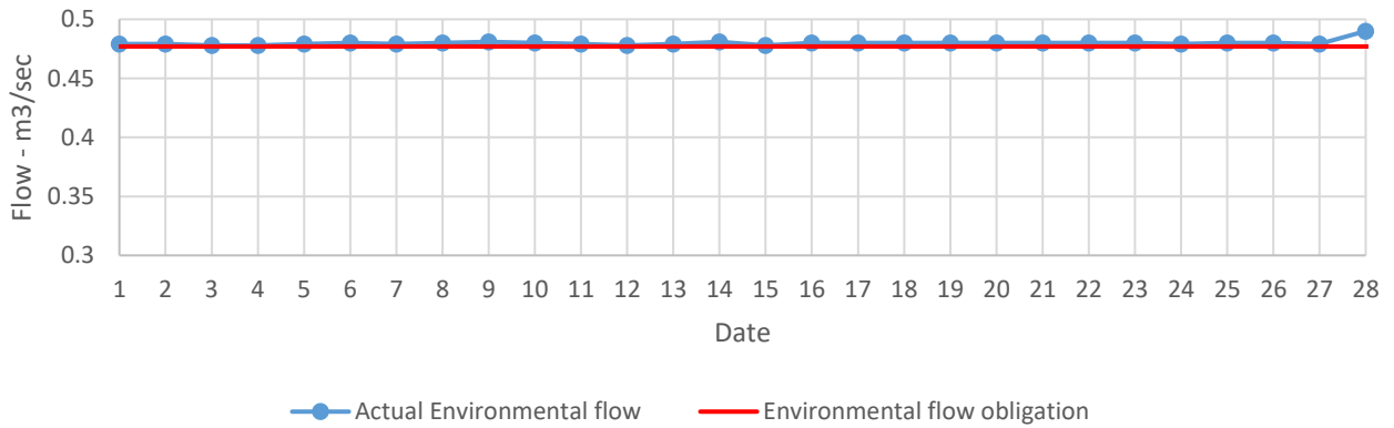
Chirukhi Environmental flow February 2023
