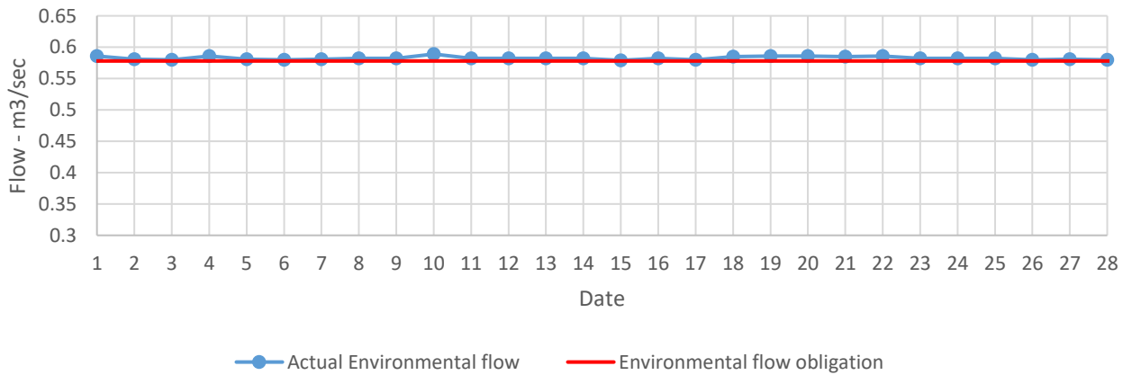
Skhalta Environmental flow February 2023
