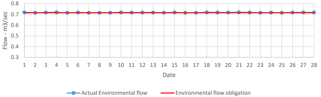
Didachara Environmental flow February 2023
