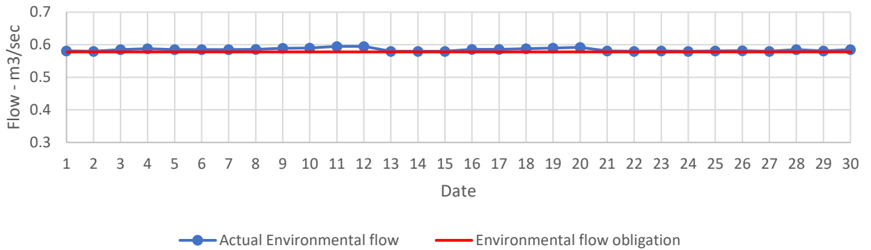
Skhalta Environmental flow April 2022
