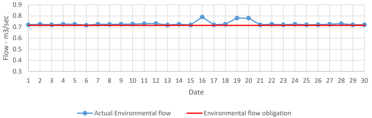
Didachara Environmental flow April 2022
