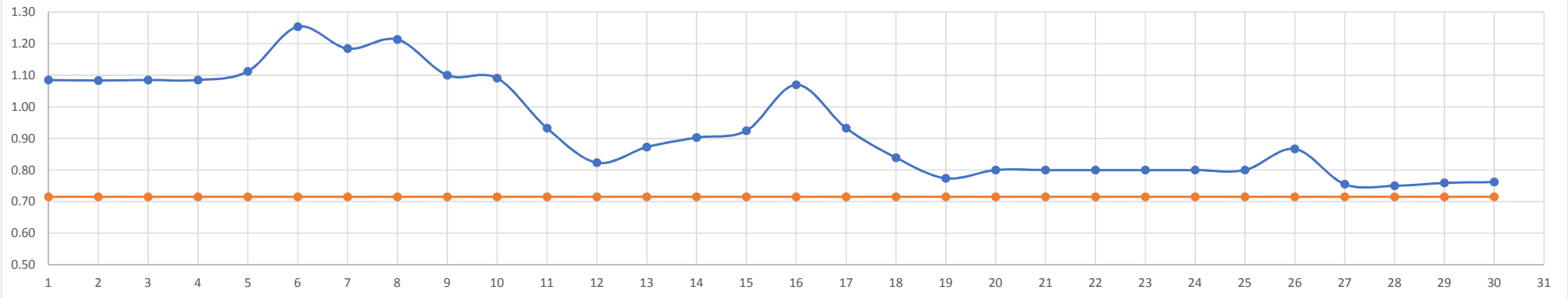
Environmental Flow for Sept 2017 Didachara Dam Required Env Flow - 0.715 CuM/Sec Actual Flow released - Day Average CuM/Sec
