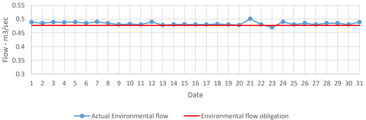
Chirukhi Environmental flow January 2024
